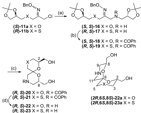
Scheme 6. Reagents and conditions: (a) MeOH, \Delta , 9c , 8 h, 61% from 11a , 67% from 11b ; (b) PhCOCl, NEt 3 , DMAP, CH 2 Cl 2 , 0 °C, 90% from 16 , 95% from 17 ; (c) Amberlyst ® 15, (CH 2 O) n , acetone/H 2 O (10:1), \Delta , 61% from 18 , 65% from 19 ; (d) LiAlH 4 , THF, nearly quantitative.
