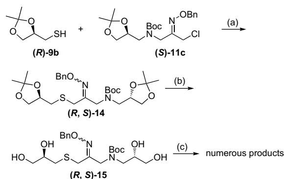
Scheme 5. Reagents and conditions: (a) KH, THF, 81%; (b) Amberlyst® 15, acetone/H 2 O (10:1), \Delta , 4 h, 33%; (c) \Delta .
